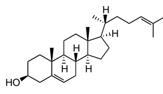
Desmosterol (24-Dehydrocholesterol)
