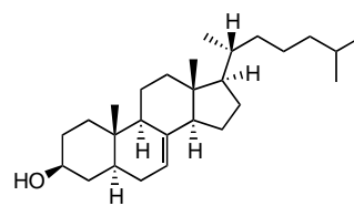
Lathosterol
