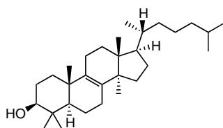
24,25-Dihydrolanosterol
