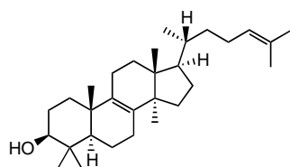
Lanosterol
