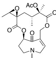
Neopetasitenine
