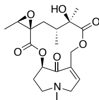
Petasitenine (Fukinotoxin)
