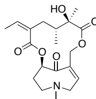
Senkirkine
