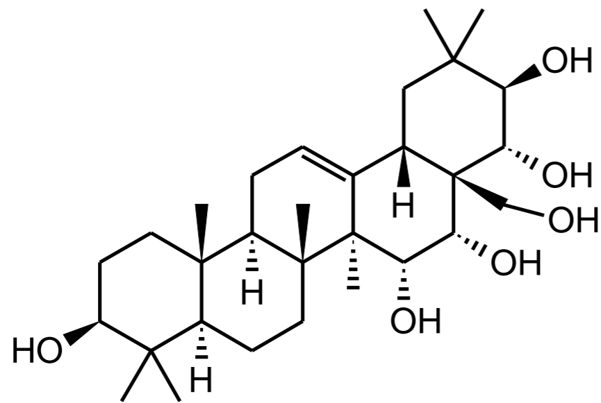
茶サポゲニン
